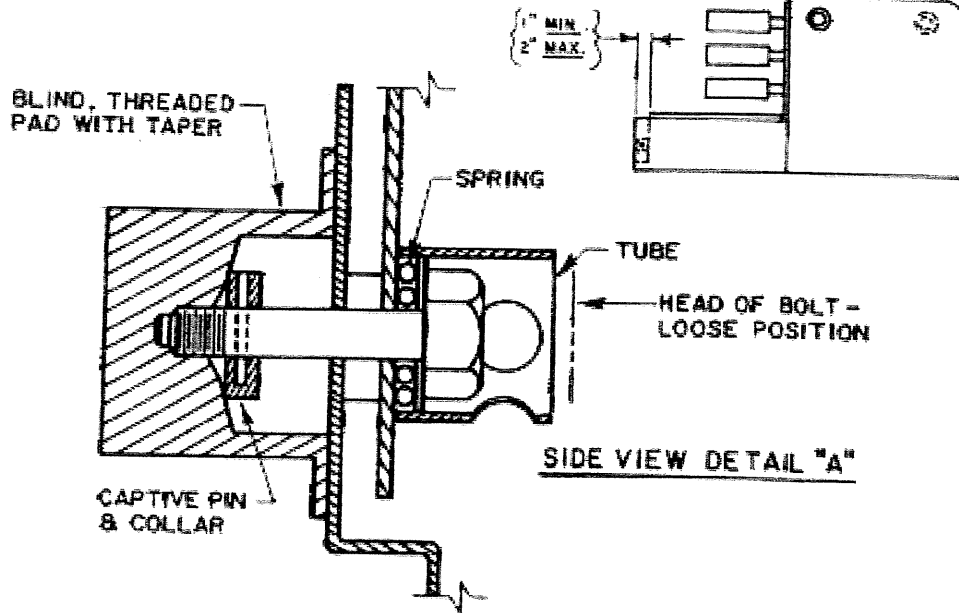
FIGURE 5 LOCKING PROVISION
