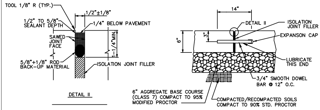
TYP. DOWELED ISOLATION JOINT (DIJ) DETAIL SCALE: NTS
