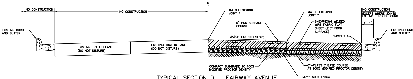
TYPICAL SECTION D – FAIRWAY AVENUE
