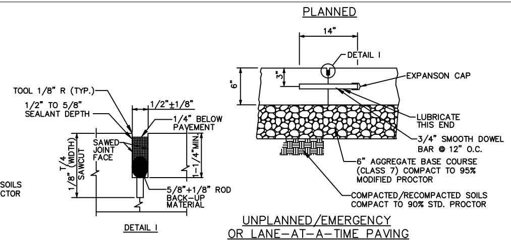
TYP. CONSTRUCTION JOINT (CJ) DETAIL SCALE: NTS
