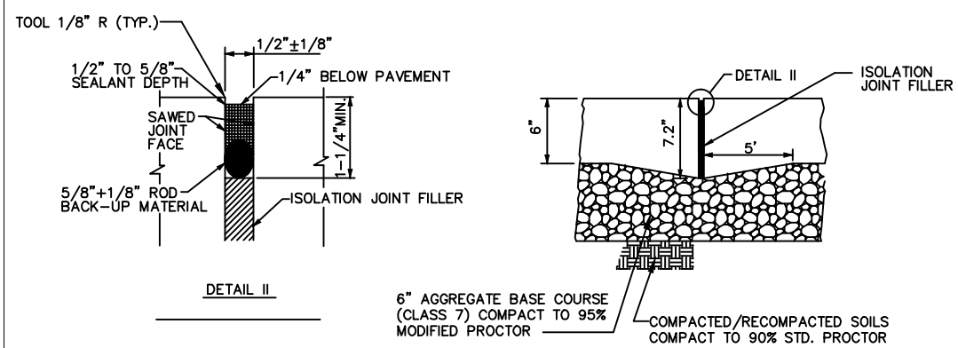
TYP. ISOLATION JOINT (IJ) DETAIL SCALE: NTS
