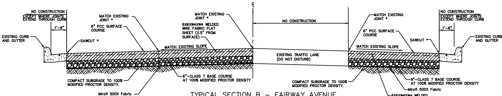
TYPICAL SECTION B – FAIRWAY AVENUE
