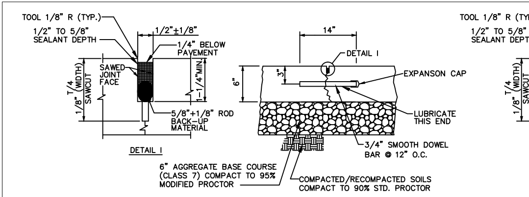
TYP. DOWELED JOINT (DJ) DETAIL SCALE: NTS
