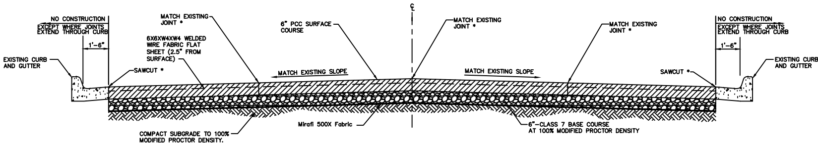
TYPICAL SECTION A – CRESTWOOD ROAD
