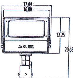
Tenon Mount Luminaire EPA of 1.89 Ft 2 and max weight 28 lbs.
