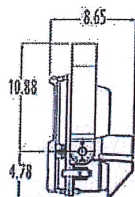
YKE-Yoke Mount Luminaire EPA of 1.76 Ft 2 and max weight 31 lbs.
