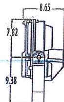
YK-Yoke Mount Luminaire EPA of 1.76 Ft 2 and max weight 30 lbs.
