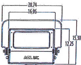
YKE-Yoke Mount Luminaire EPA of 1.76 Ft 2 and max weight 31 lbs.
