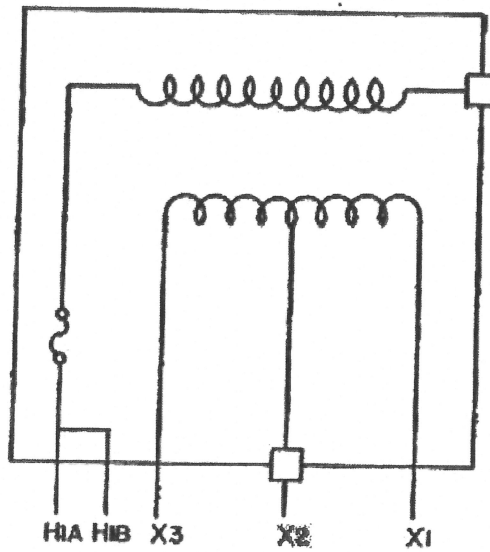
FIGURE 3 INTERNAL CONNECTIONS & TERMINAL DESIGNATIONS
