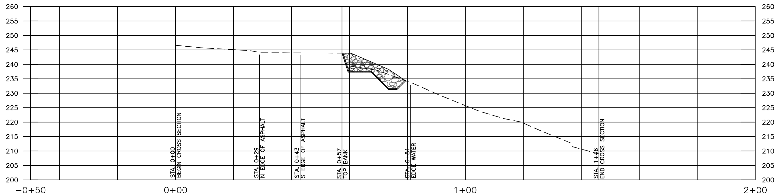
CROSS SECTION 2
