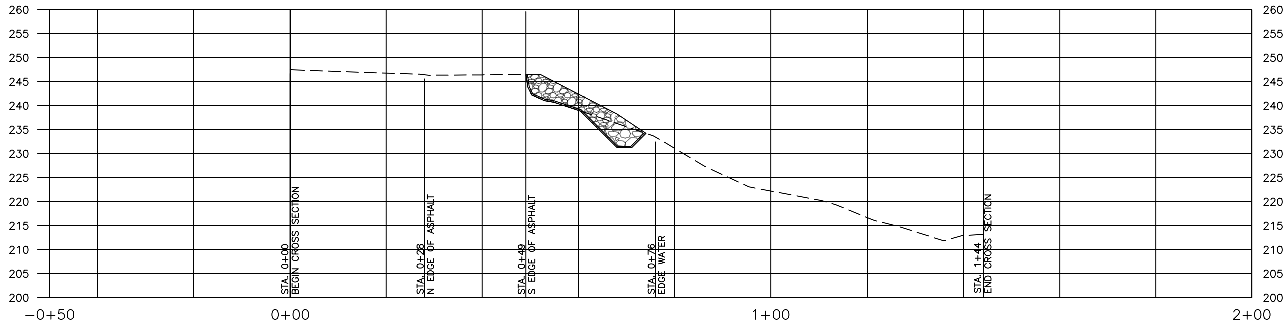
CROSS SECTION 3
