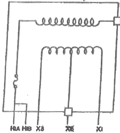
FIGURE 3 INTERNAL CONNECTIONS & TERMINAL DESIGNATIONS
