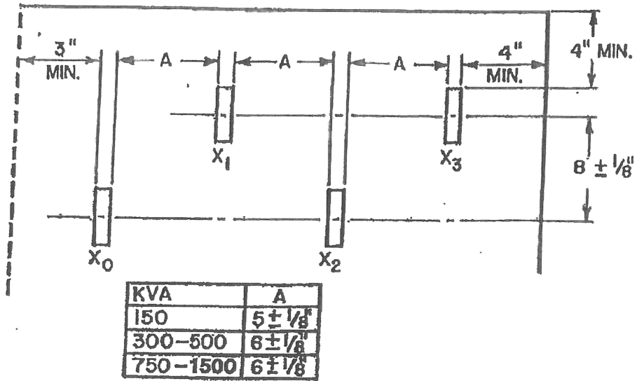
LOW VOLTAGE BUSHING TERMINALS AND ARRANGEMENTS
